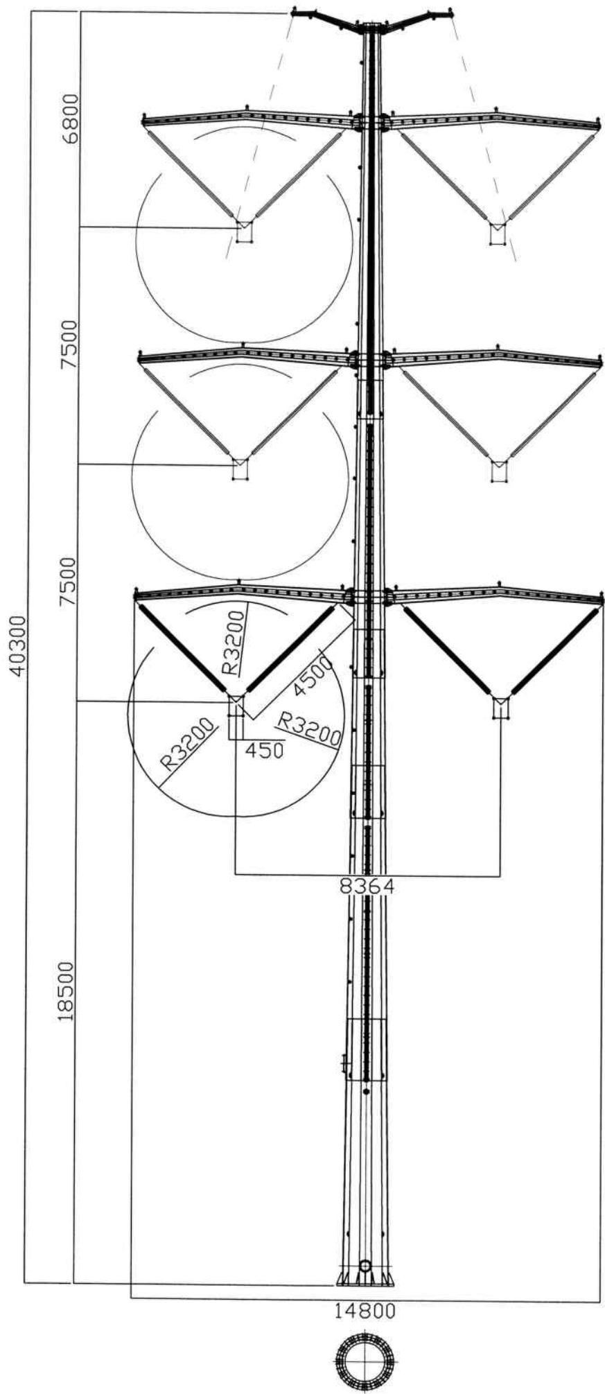
400kV DOUBLE CIRCUIT CONCEPTUAL MONOPOLE
