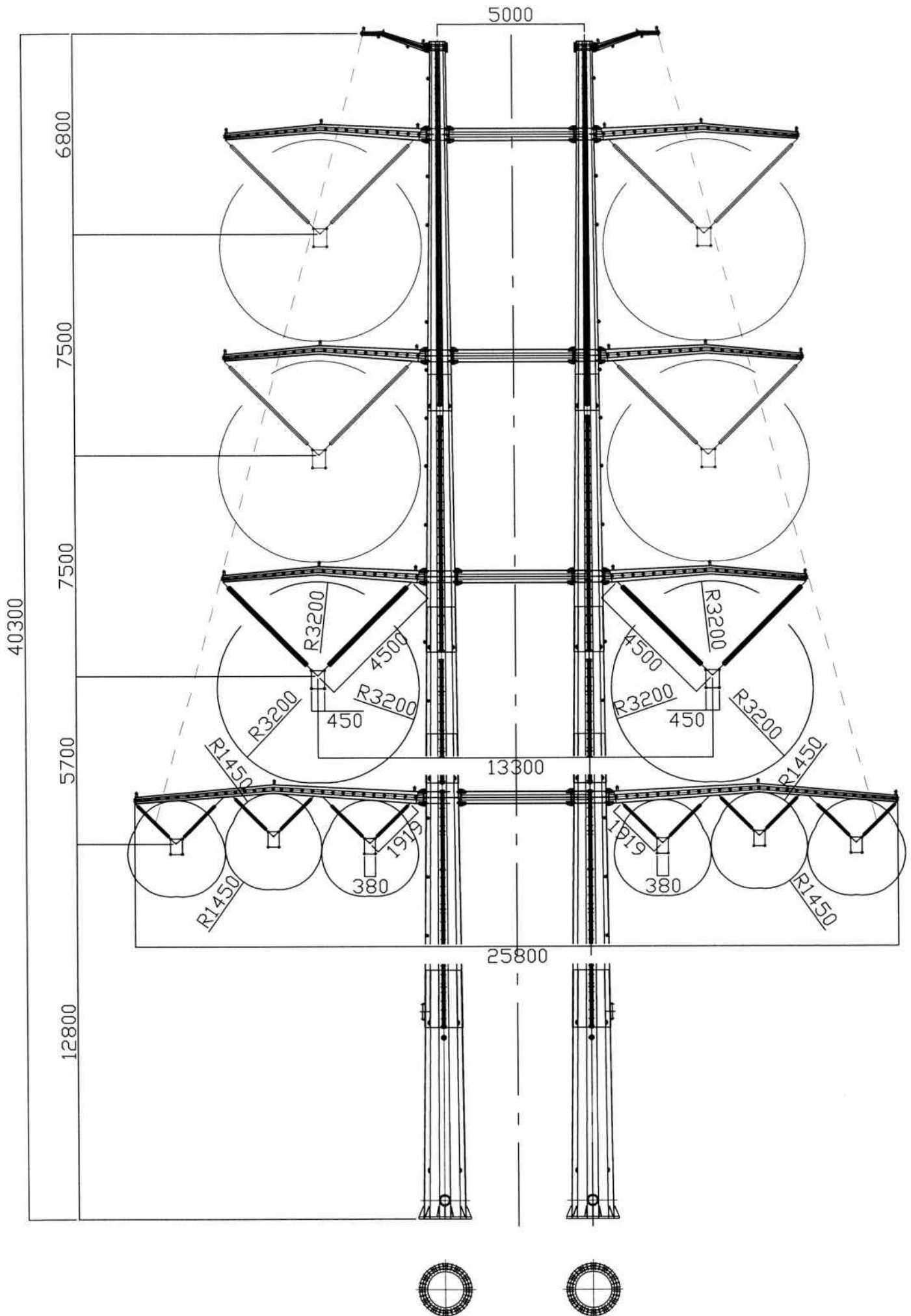
400kV & 132kV DOUBLE CIRCUITS CONCEPTUAL DOUBLE MONOPOLE
